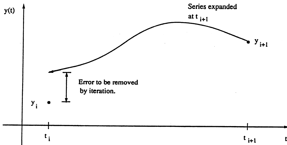
Figure 3: Implicit \sigma Taylor series method
